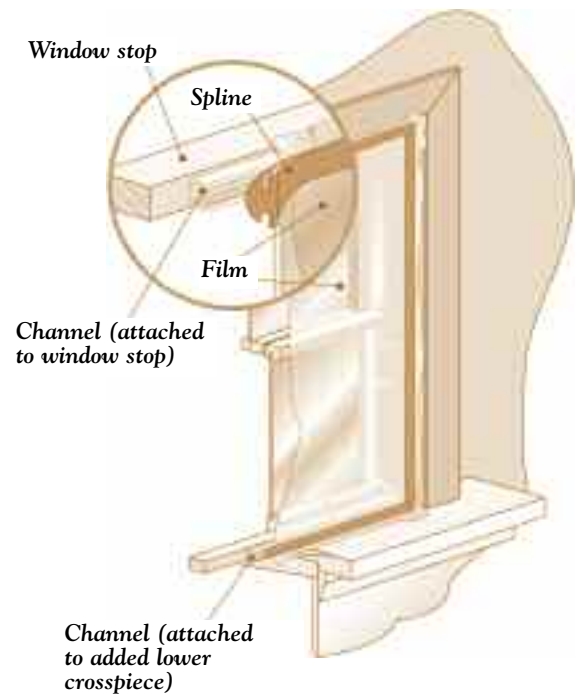
Figure 8 Clear plastic film with spline and channel
