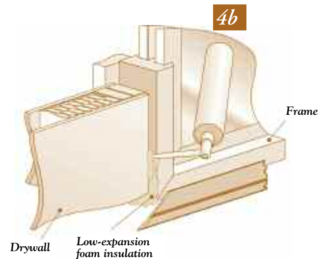
Figures 4a and 4b ..... How to seal behind the window trim
